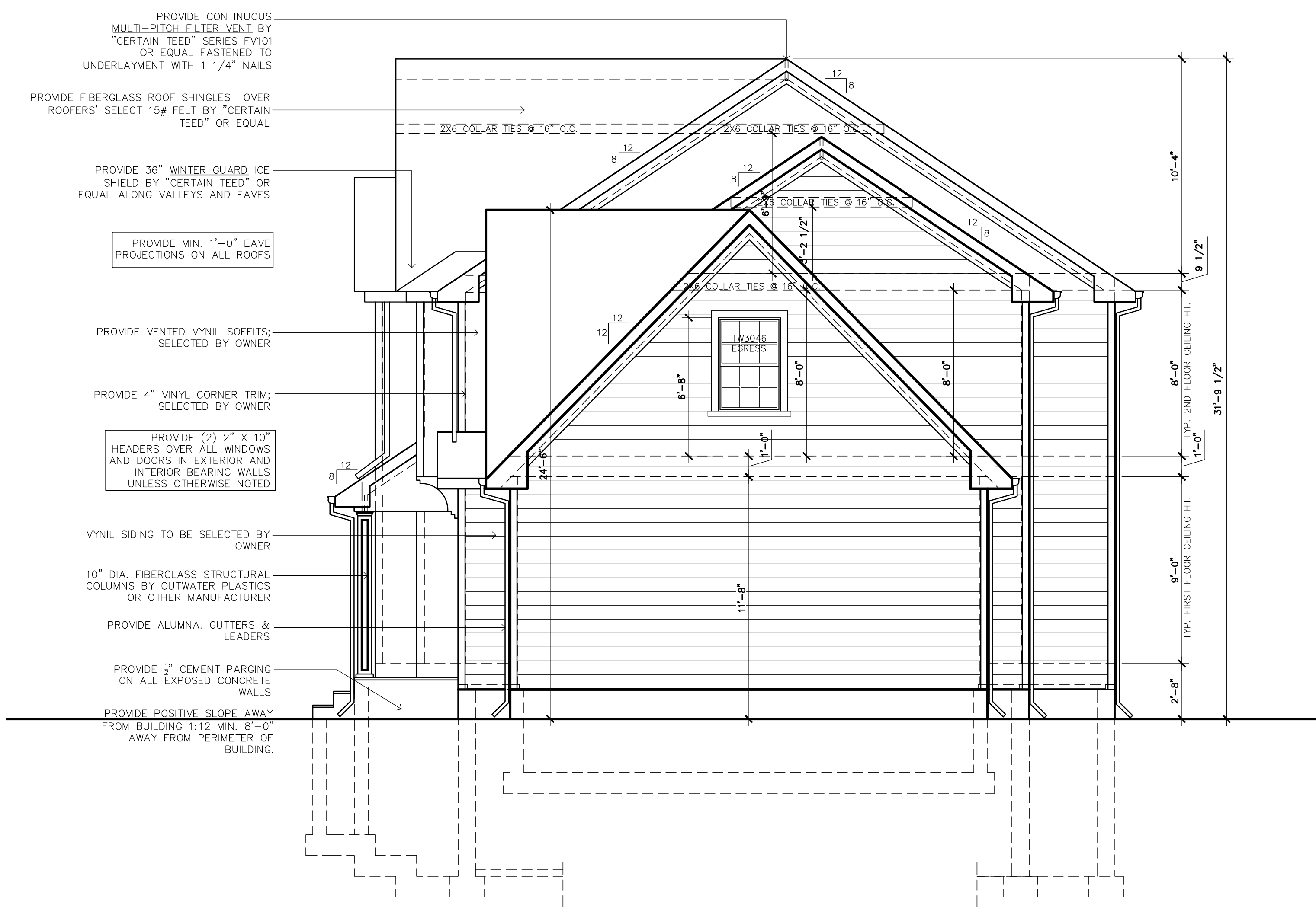
1 RIGHT SIDE ELEVATION 1/4" = 1'-0"
