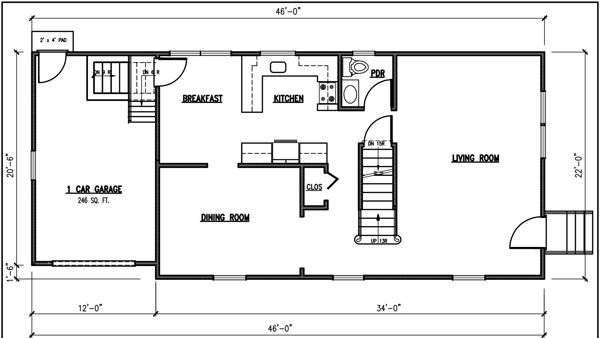
FIRST FLOOR PLAN 748 SQ. FT.
