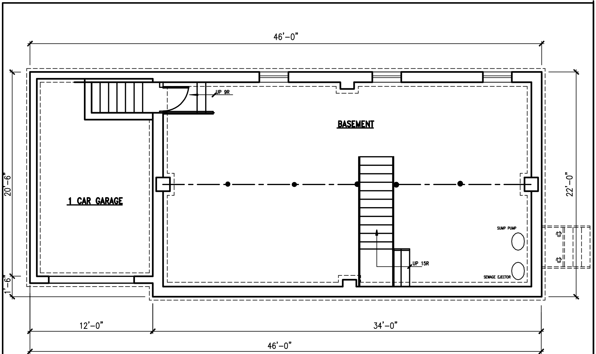
FOUNDATION/BASEMENT PLAN 994 SQ. FT. FOOT PRINT
