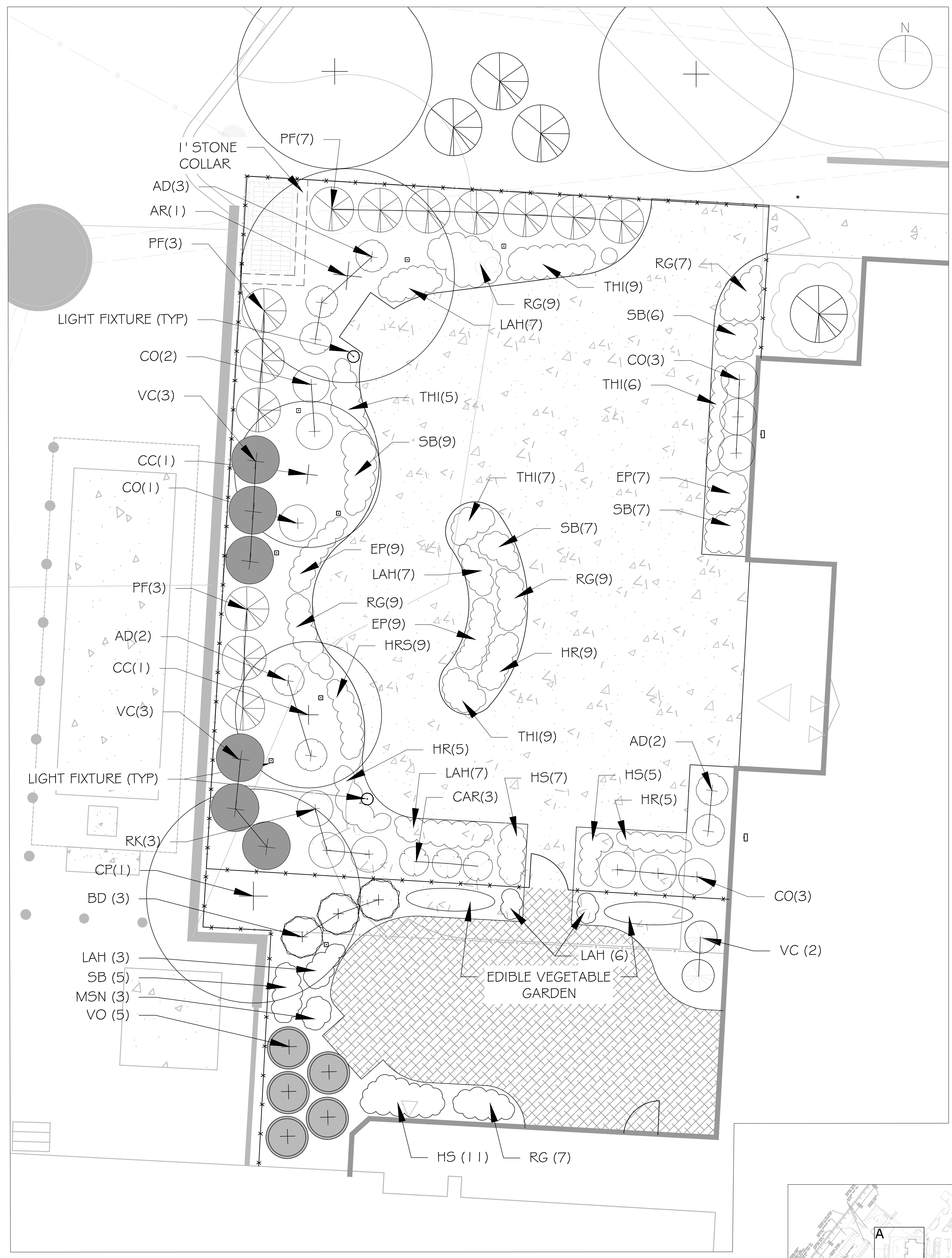
A COURTYARD AREA A SCALE: 1"=5'
