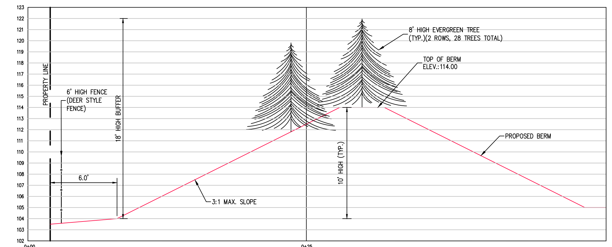
SECTION A - A SCALE: HORIZONTAL - 1"=5' VERTICAL - 1"=5'
