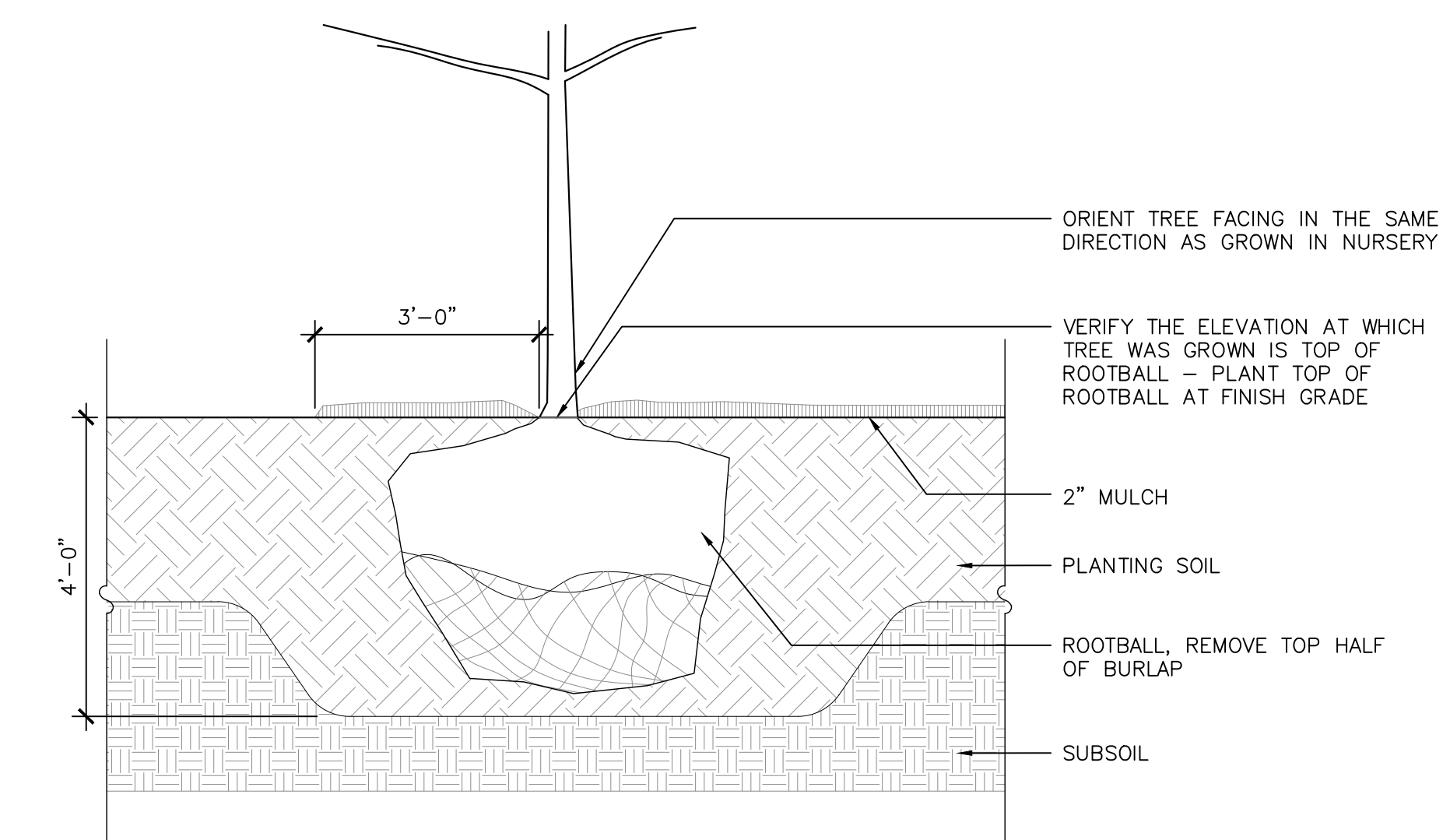
1 TREE PLANTING, TYP. 1/8" = 1'-0"
