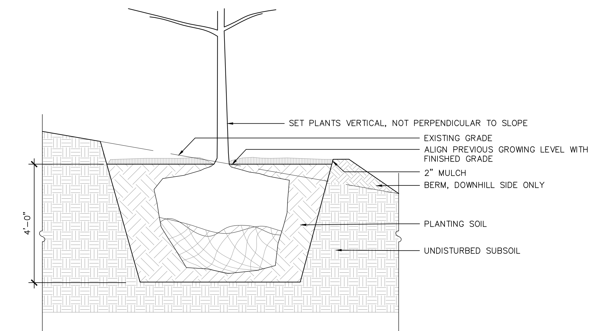
2 TREE PLANTING ON SLOPE, TYP. - SECT 1/8" = 1'-0"
