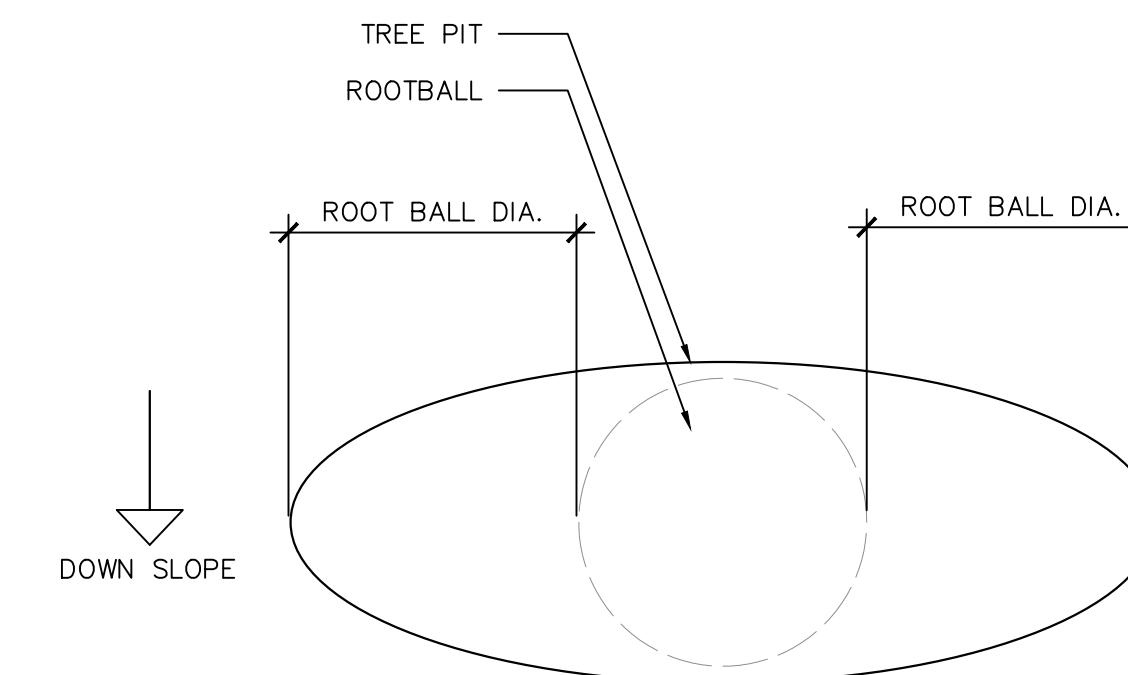
3 TREE PLANTING ON SLOPE, TYP. - PLAN N.T.S.
