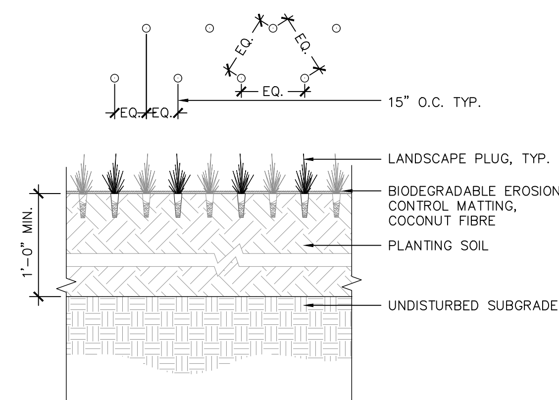
5 LANDSCAPE PLUG PLANTING, TYP. 1" = 1'
