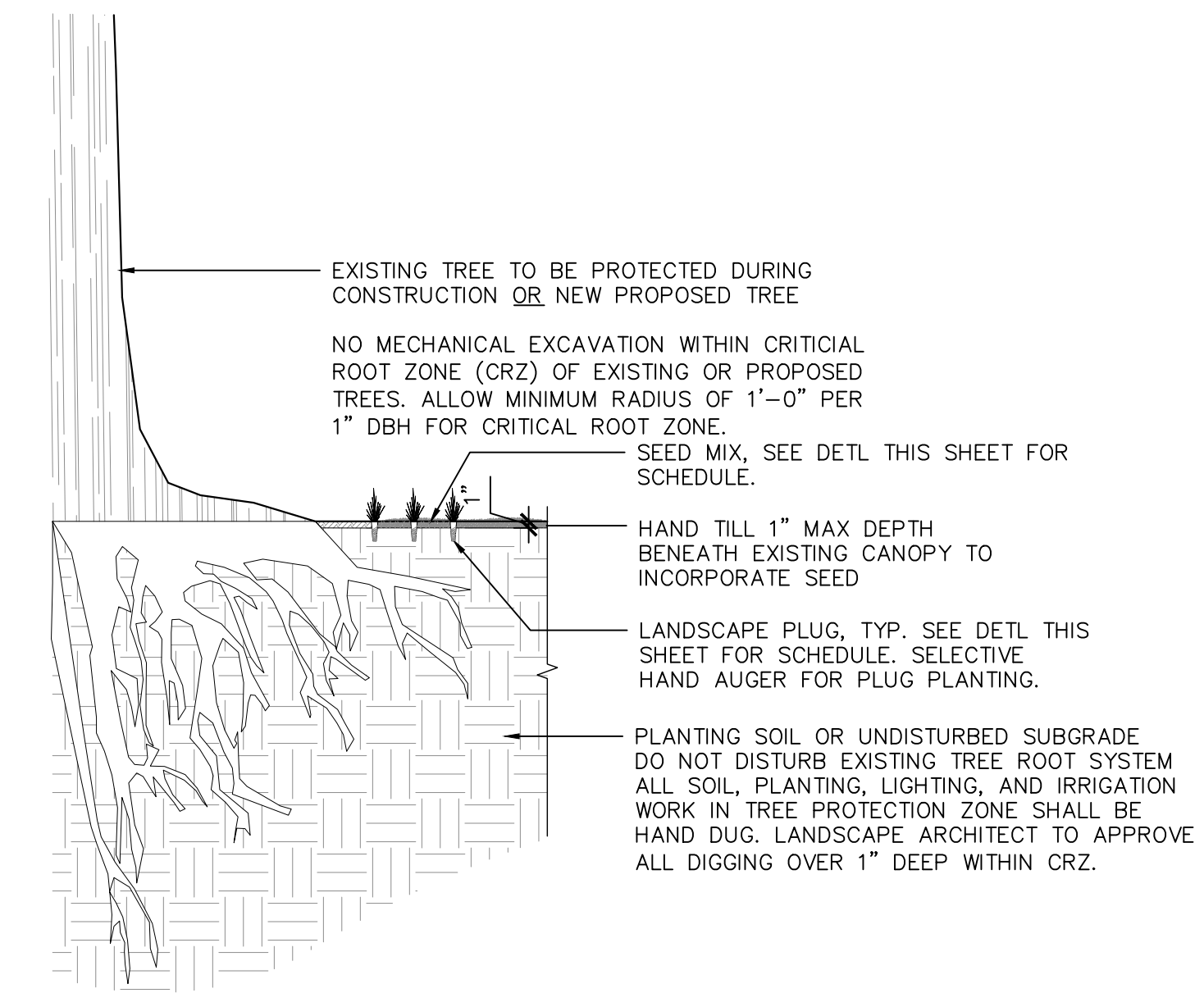
4 SEED/PLUG PLANTING @ TREE, TYP. 1/8" = 1'-0"
