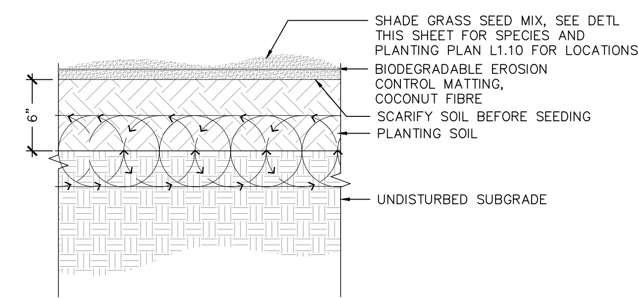
6 SEED PLANTING, TYP. 1" = 1'
